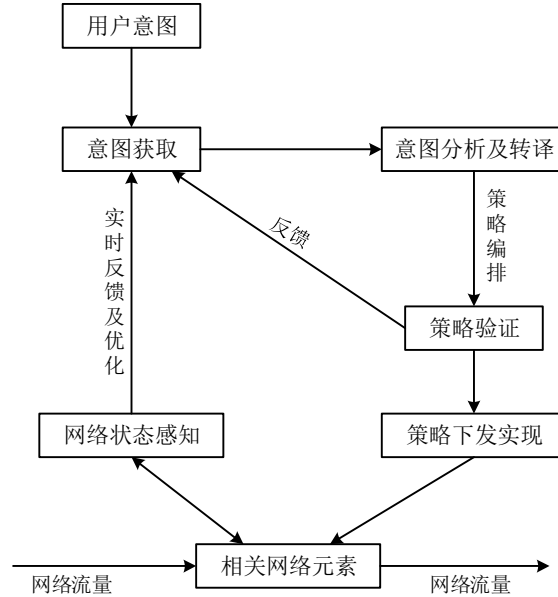
Fig.2 Implementation process of IBN
