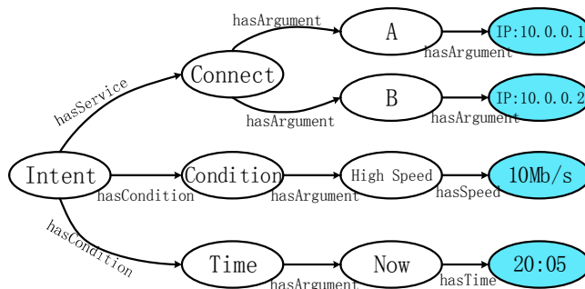
Fig.3 Using RDF Graph to describe intent
