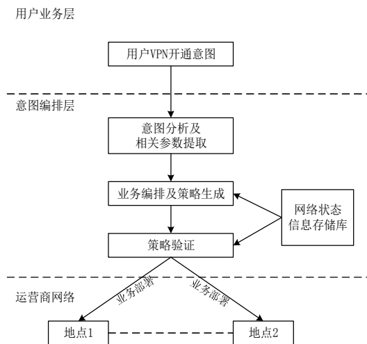
Fig.6 Implementation process of Intent Driven VPN deployment
