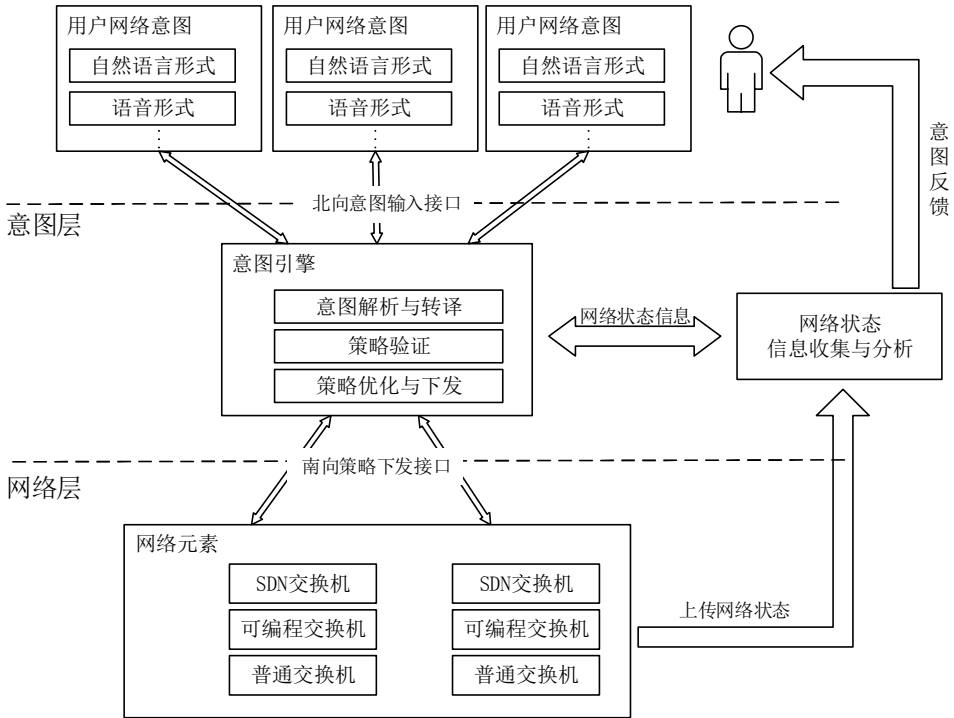
Fig.1 IBN architecture
