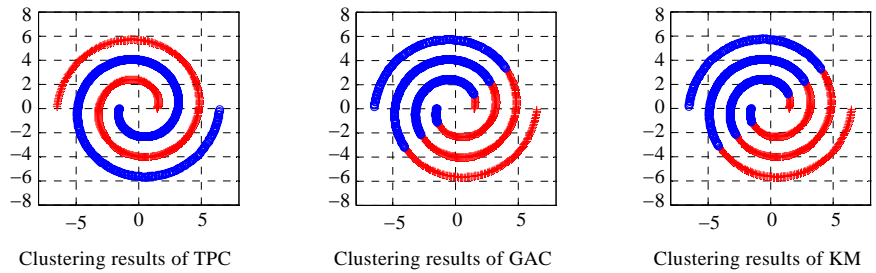
(b) Typical clustering results on Spiral obtained from three algorithms (b) 3种算法对数据集 Spiral 的典型聚类结果
