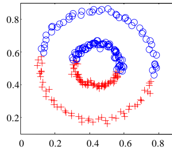
Fig.1 Euclidian distance metric cannot reflect the global consistency of the data set
