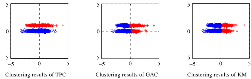
(a) Typical clustering results on Long1 obtained from three algorithms (a) 3种算法对数据集 Long1 的典型聚类结果
