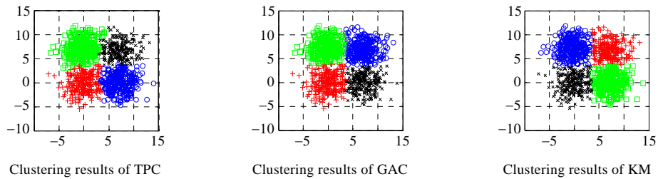
(b) Typical clustering results on Square4 obtained from three algorithms
