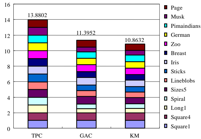
Fig.6 Comparison of robustness of three algorithms
