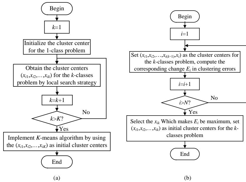
Fig.2 Flow chart of global selection strategy 图 2 全局选点策略的流程图
