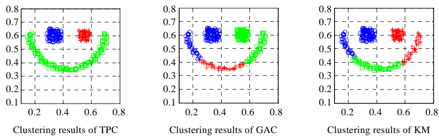
(c) Typical clustering results on Lineblobs obtained from three algorithms (c) 3种算法对数据集 Lineblobs 的典型聚类结果
