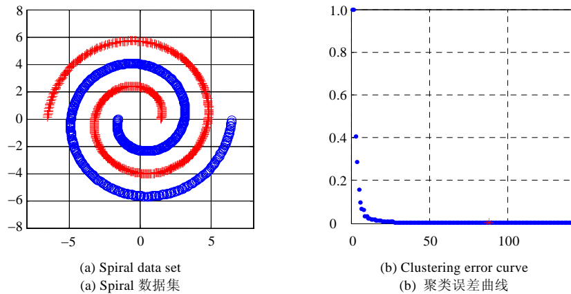
Fig.3 Adaptive selection of the number of clusters for Sporal data set
