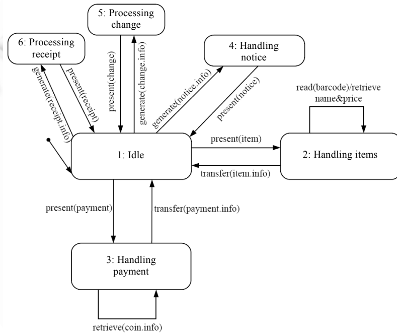
Fig.9 State-Diagram for POS domain
