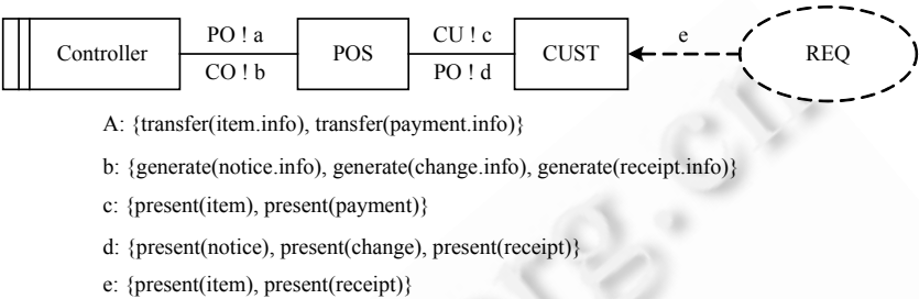
Fig.7 Problem diagram of self-help point-of-sale system 图 7 自助式销售点系统问题图
