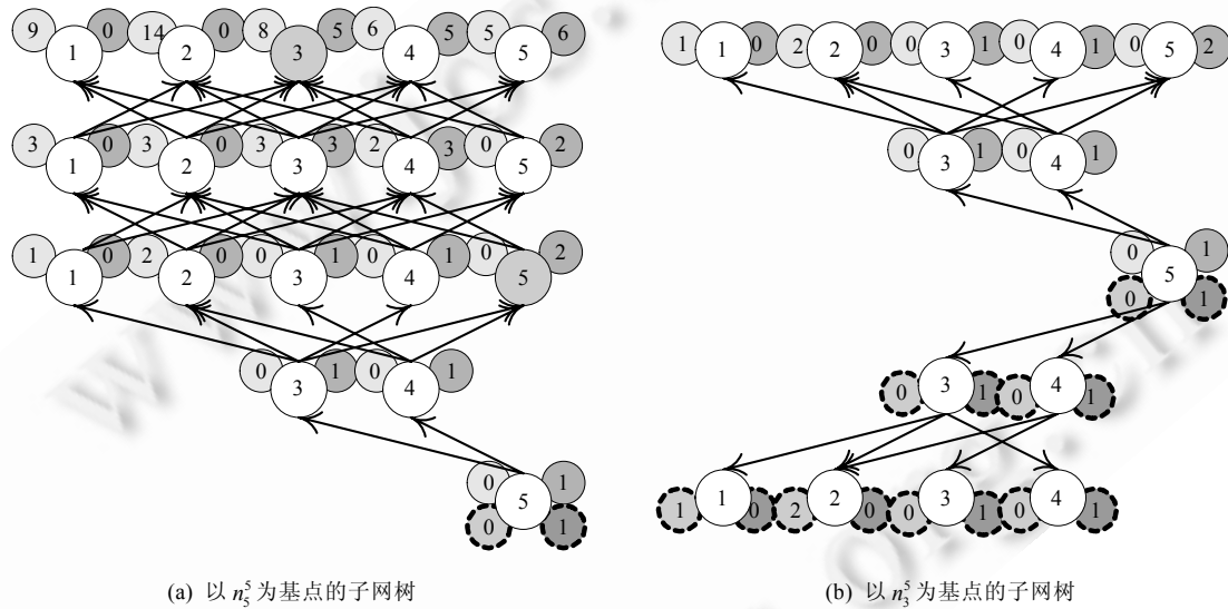
Fig.2 Some Subnettrees of including 5
