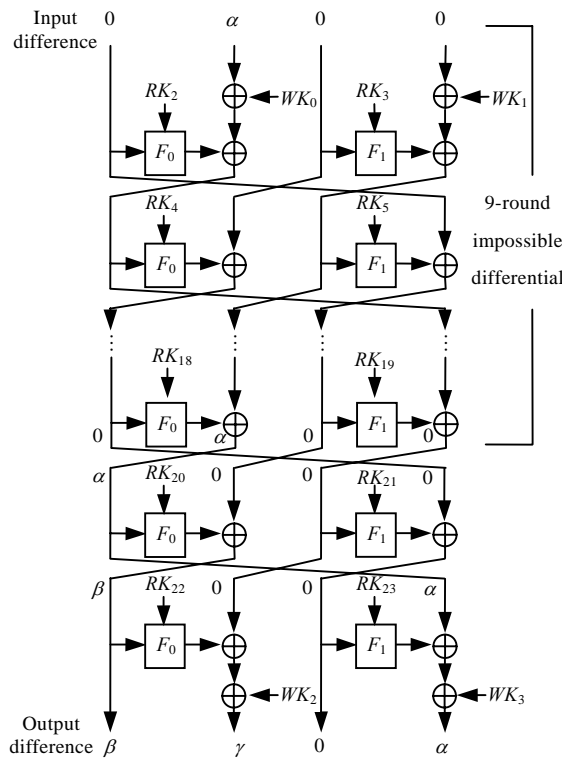
Fig.3 Impossible differential attack on 11-round CLEFIA
