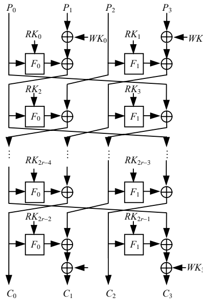
Fig.1 Encryption process of r -round CLEFIA
