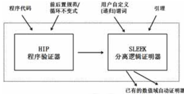
Fig.3 HIP/SLEEK: Automated program verification via separation logic
