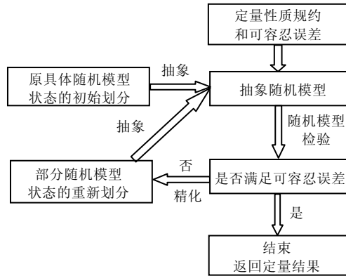
Fig.4 Error guided abstraction-refinement
