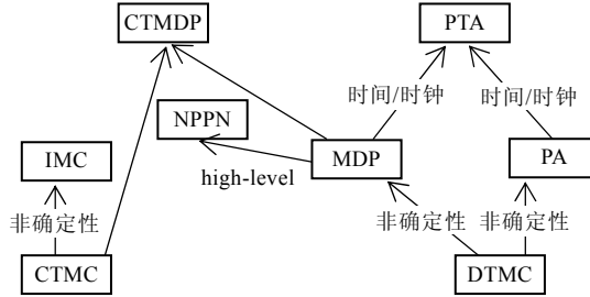
Fig.1 Relationship among stochastic system models 图 1 随机系统模型间的关系
