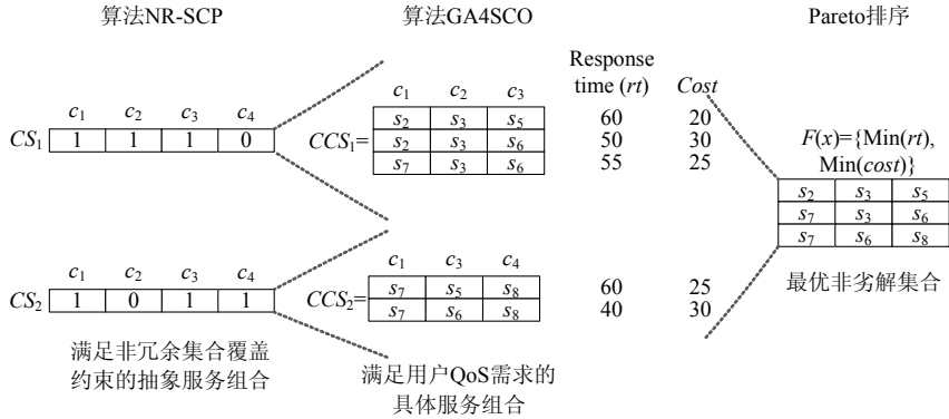
Fig.8 Merging and ranking of local optimization results
