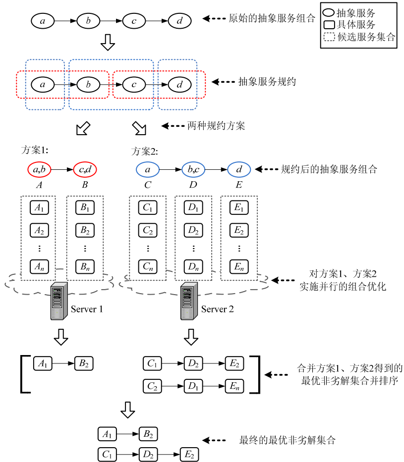
Fig.2 Service selection approach based on functionality folding
