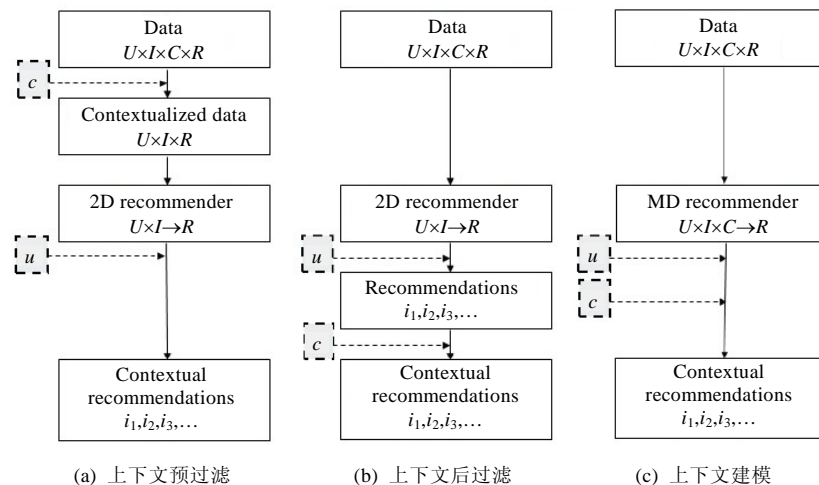
Fig.2 Adomavicius-Tuzhilin classification [8]
