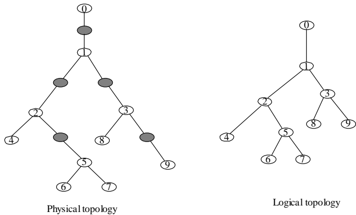
Fig.12 Physical topology and logical topology
