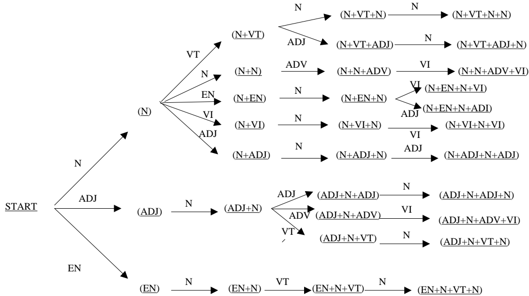
Fig.1 The DFA representation of the right syntax pattern of seven character sentence 图 1 七字词句合法句法模式的 DFA 表示
