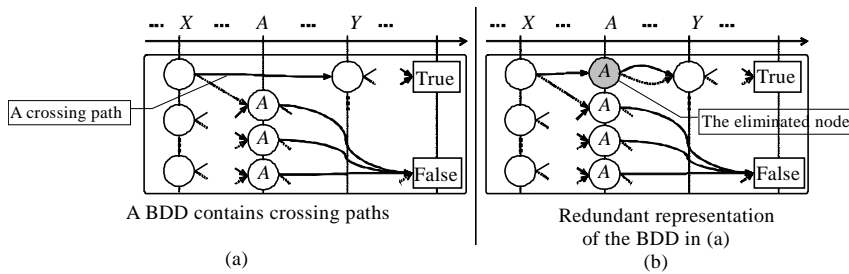
Fig.3 Crossing paths in BDD and their redundant representations
