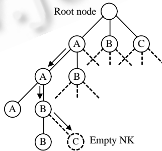
Fig.3 Node with original NK of AABB* being AABC
