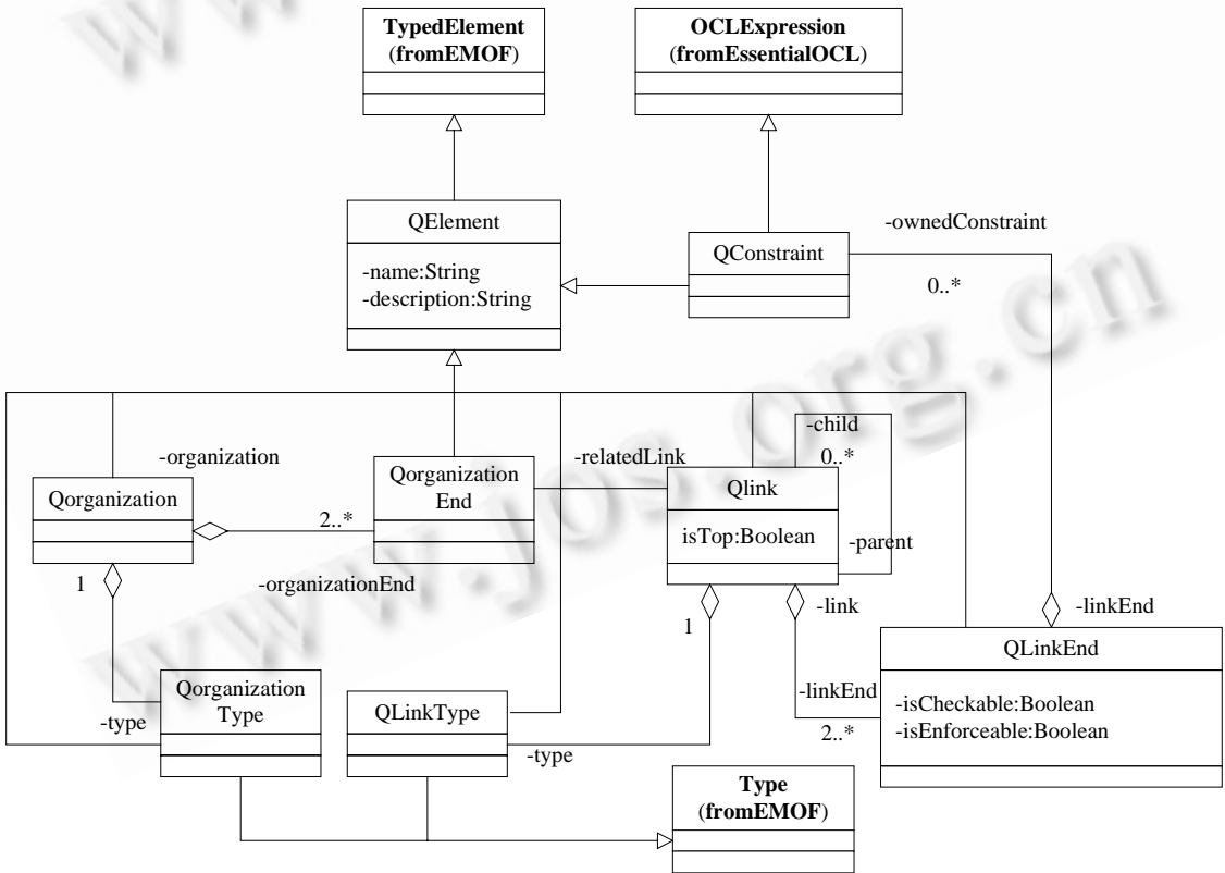
Fig.4 The part 2 of metamodel diagram of QMTW
