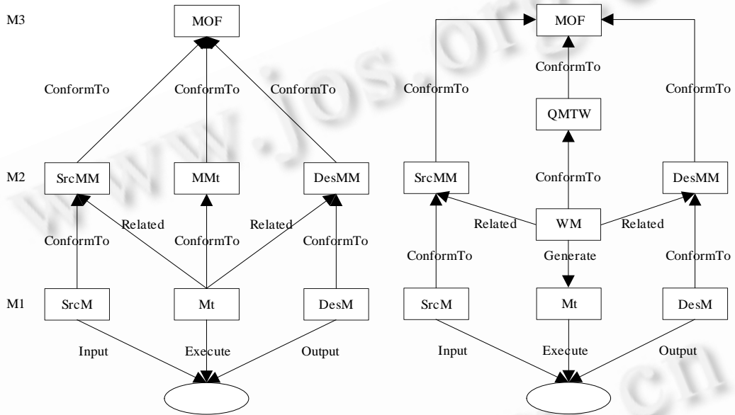
Fig.1 Comparison between model transformation layers and QMTW layers
