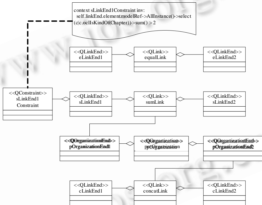
Fig.6 Book2Publication weaving model instance diagram—Link and organization 图 6 Book2Publication 编织模型实例图——连接与组织
