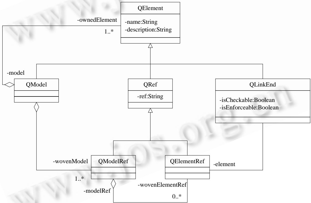
Fig.3 The part 1 of metamodel diagram of QMTW
