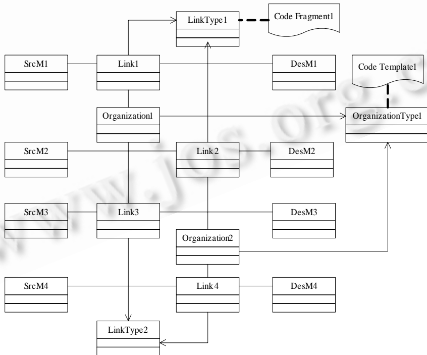
Fig.2 Model transformation weaving sketch map
