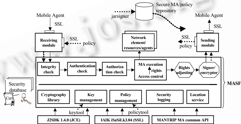
Fig.2 The architecture of mobile Agent security facility 图 2 移动 Agent 安全设施的体系结构
