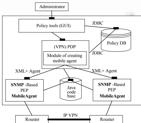
Fig.1 Network management based on the mobile Agent and the policy
