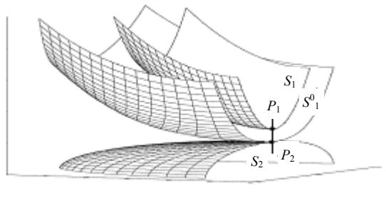
Fig.1 An example of topology transition point
