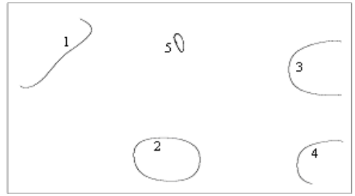
Fig.6 h=-1, l=-0.5 , 2nd and 4th together with 5th TTP create 1 st intersection loop, 1st and 6th TTP create enclosed intersection loop, 2nd and 3rd TTP create 3rd and 4th open curves
