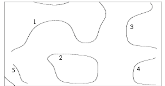
Fig.10 h=0.7, l=0.35 , 10th TTP merge 5th and 6th intersection curve into 5th intersection curve
