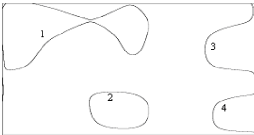
Fig.7 h=0, l=0 , 7th TTP merge 1st and 5th curve into 1 intersection curve
