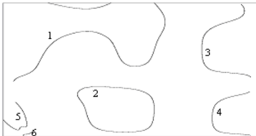
Fig.9 h=0.6, l=0.3 , 9th TTP creates 6th open curve
