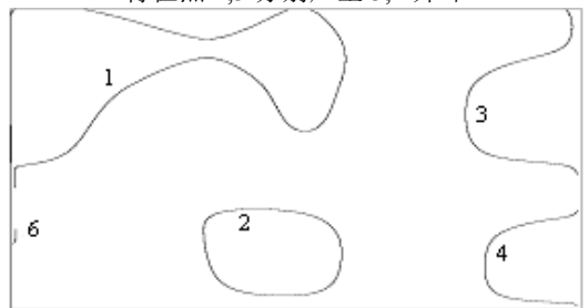
Fig.8 h=0.1, l=0.05 , 8th TTP create 5th open curve
