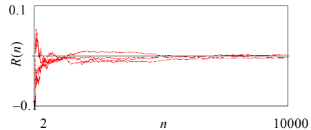
Fig.2 Correlation degree function R(x_0, n) of different key x_0
