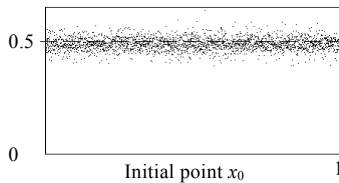
Fig.1 The distribution of \alpha(M, x_0, n) , where n=10000, M=0^n
