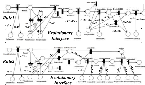
Fig.10 Adaptive strategy Petri net model
