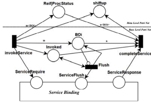
Fig.6 Business operation Petri net model
