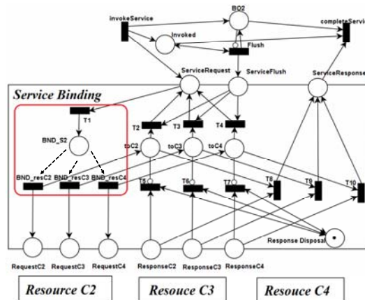
Fig.8 Binding between business operation with resource PN model
