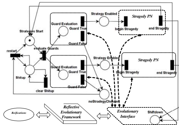
Fig.9 Adaptive strategy structure Petri net model
