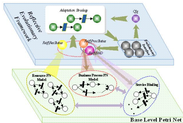
Fig.4 Reflective Petri net based ASBS performance model
