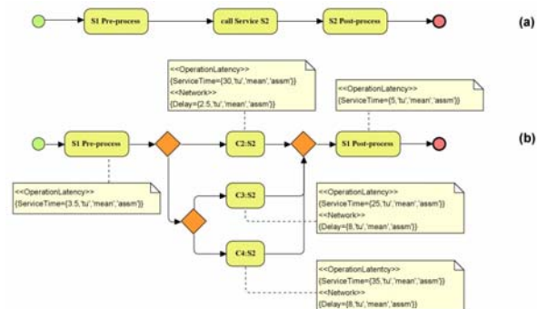
Fig.2 (a) Business workflow (b) Business workflow with resource description
