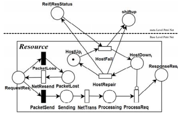
Fig.7 Resource Petri net model
