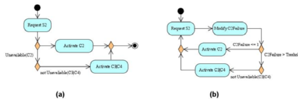
Fig.3 Adaptive strategy description
