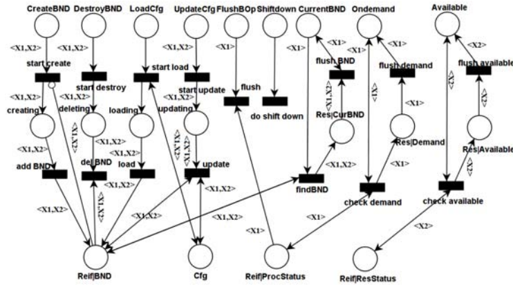
Fig.5 Reflective Petri net framework
