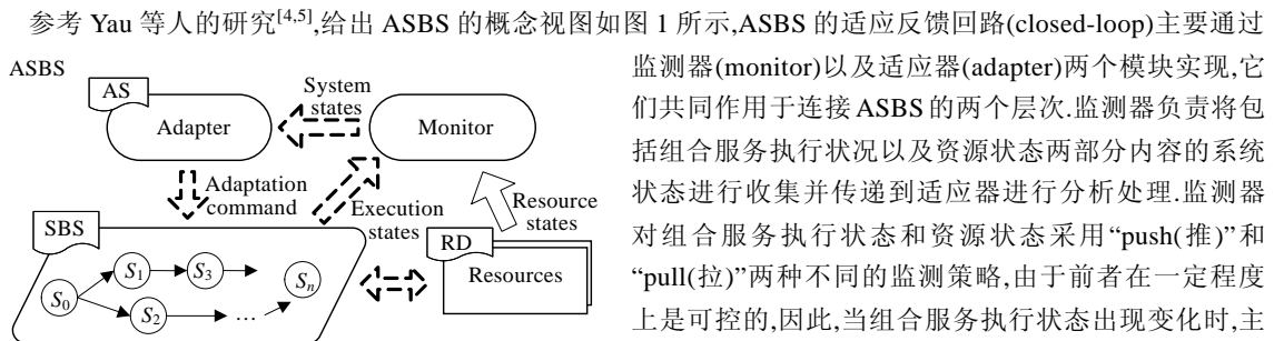
Fig.1 Conceptual view of ASBS
