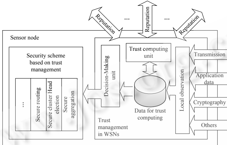
Fig.1 General architecture of trust management systems for WSNs
