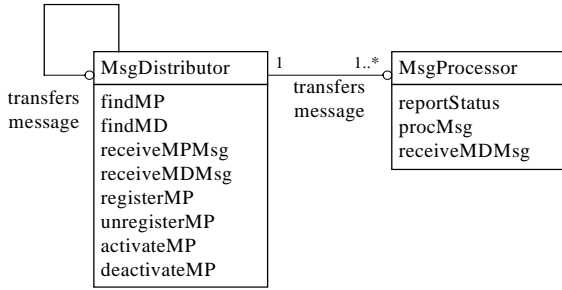
Fig.5 Class diagram of software architecture "1 MD-n MP"
