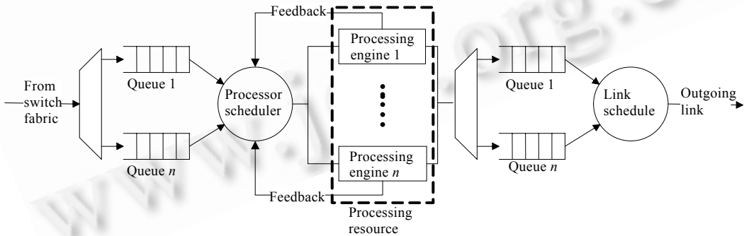
Fig.7 Packet processing system outline
