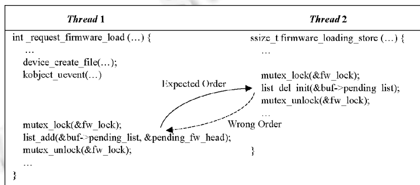
Fig.5 An example of order violation in Linux kernel v3.11.10
