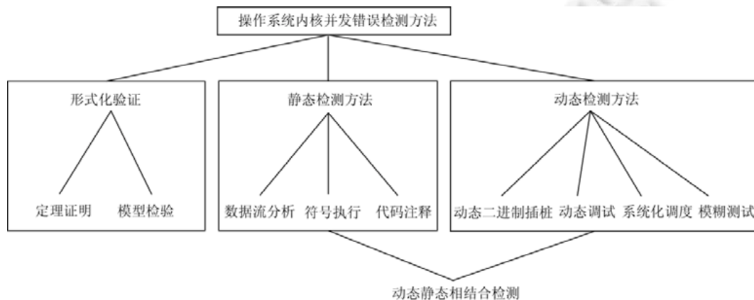
Fig.8 Approaches for concurrency bug detection in OS kernels
