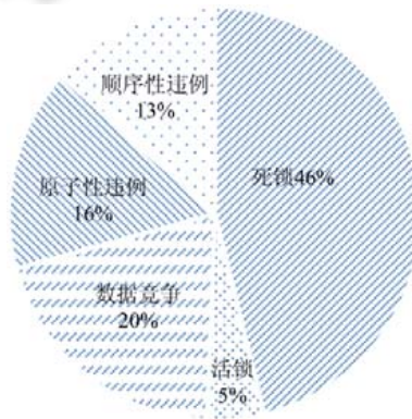
Fig.7 Distribution of concurrency bugs over categories in Linux kernel (2011~2019)
