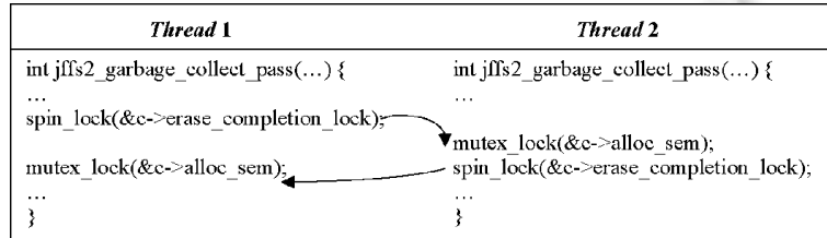
Fig.2 An example of deadlock in Linux kernel v3.0.32
