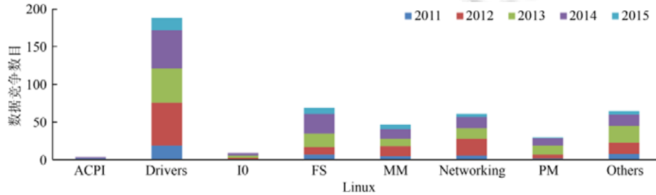
Fig.6 Distribution of data races in Linux kernel modules (2011~2015)
