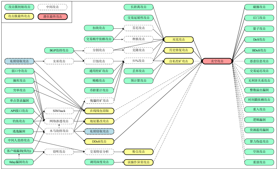
Fig.5 Associations view between block-chain attacks
