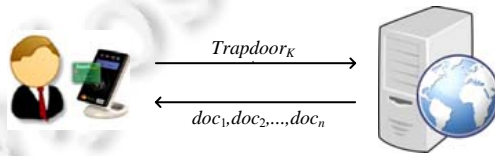
Fig.1 Threat model [4]
