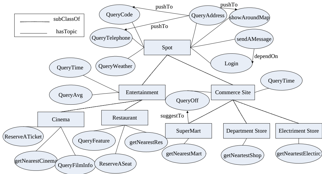
Fig.3 The snippet of SRO
