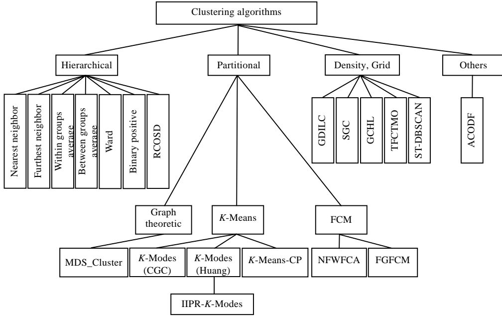
Fig.1 The classification chart of clustering algorithms
