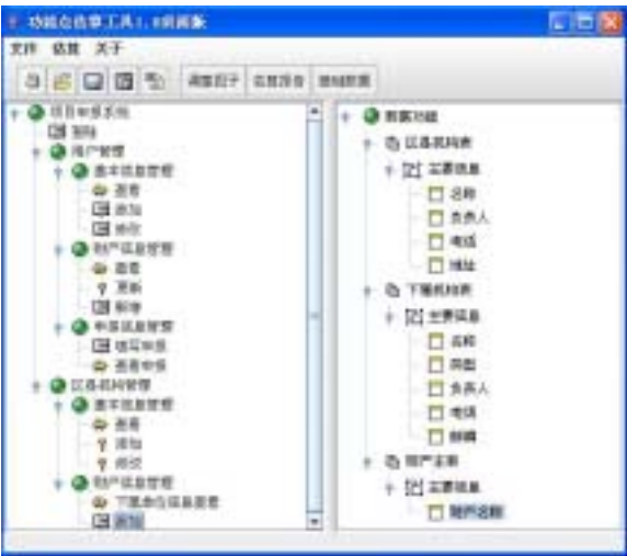
Fig.5 Software sizing in “Declaration and Management System for Government Sponsored Projects”
