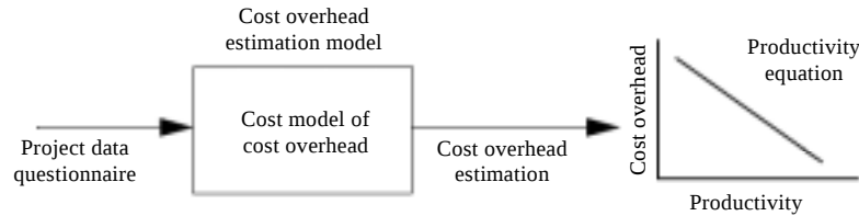
Fig.3 Overview of productivity estimation model [34]
