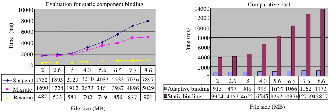
Fig.8 Performance with static application bindings
