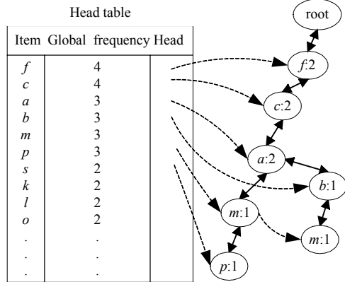
Fig.1 The frequent pattern tree on DB^1 (FP-tree(DB^1))
