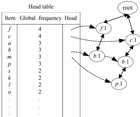
Fig.2 The frequent pattern tree on DB^2 (FP-tree(DB^2))
