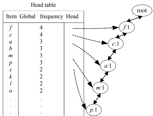
Fig.3 The frequent pattern tree on DB^3 (FP-tree(DB^3))
