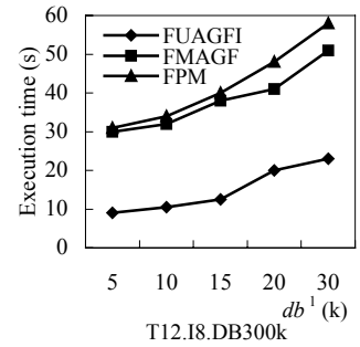
Fig.6 Execution time ( minsup=1\% )
