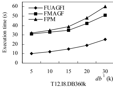
Fig.7 Execution time ( minsup=1\% )
