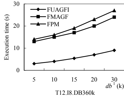
Fig.8 Execution time ( minsup=2\% )
