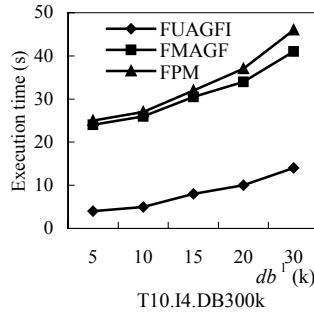
Fig.5 Execution time ( minsup=1\% )
